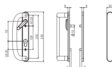
3. Internal PZ with lever/External blank
