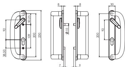
1. Internal PZ with lever/External PZ with lever
