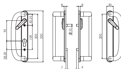
2. Internal PZ with lever/External blind with lever
