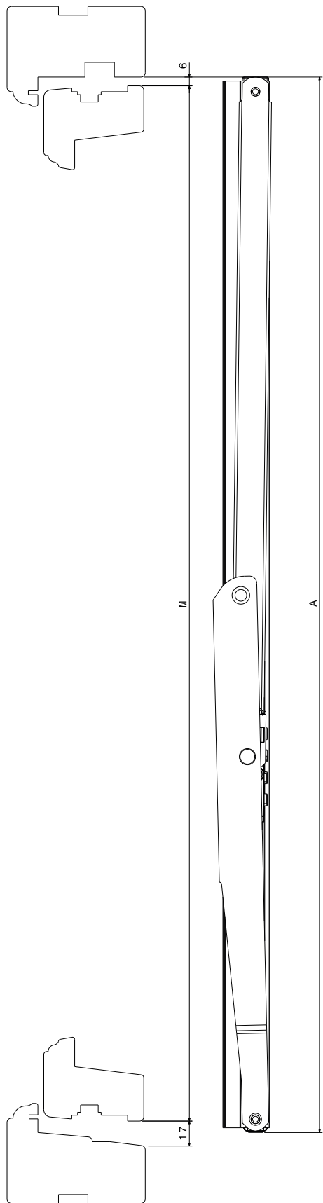
System 2000 HS1 Fully Reversible Detail
