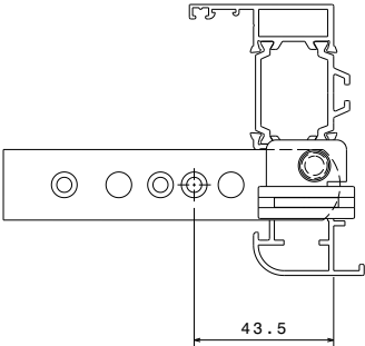
Top Bracket Fixing Position
