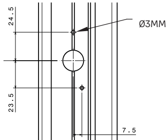
Sash Casting Fixing Hole Positioning
