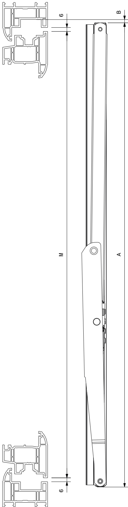
Sash Casting Fixing Hole Positioning
