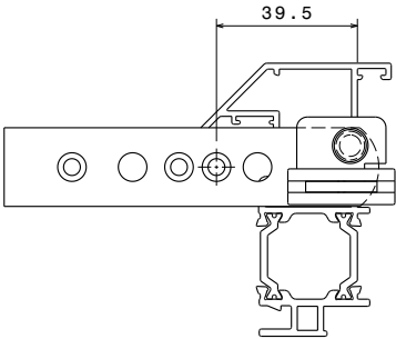
Top Bracket Fixing Position
