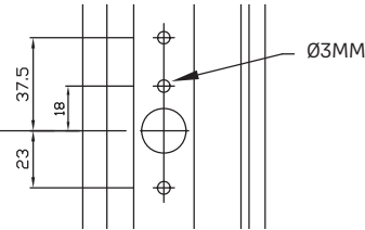
Sash Casting Fixing Hole Positioning
