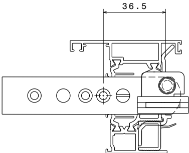
Top Bracket Fixing Position
