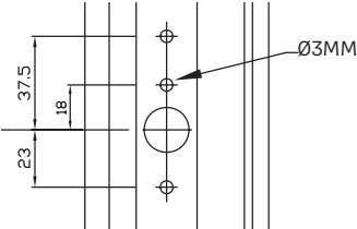
Sash Casting Fixing Hole Positioning
