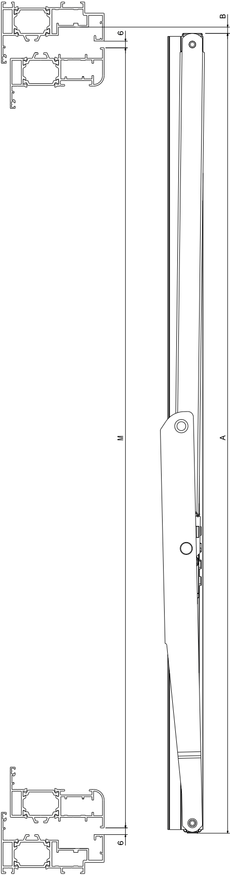
Senior Architectural Systems SPW600e Fully Reversible Detail
