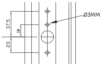
Sash Casting Fixing Hole Positioning
